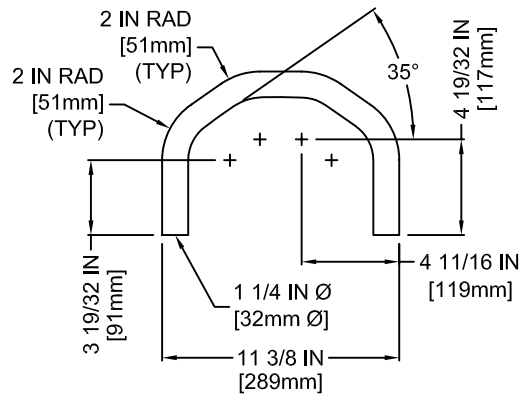
HOOK DETAIL
