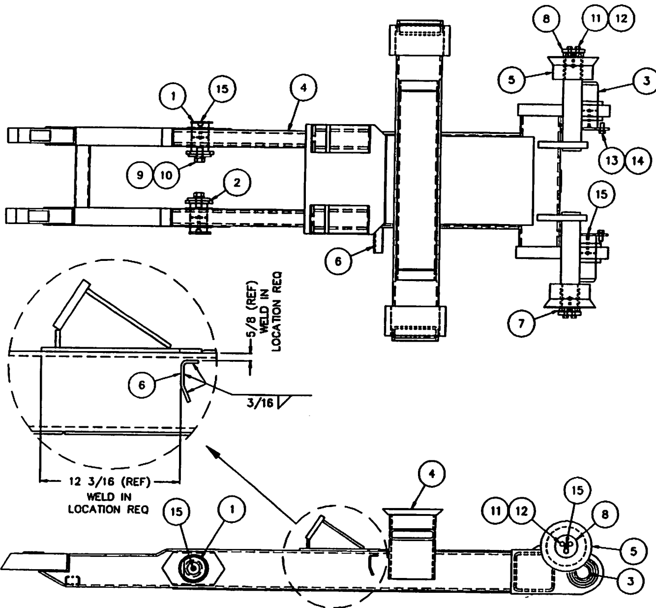
PIVOT JOINT SUB-ASSEMBLY SL-545/405 DWG.-40H96 ~ REV A
