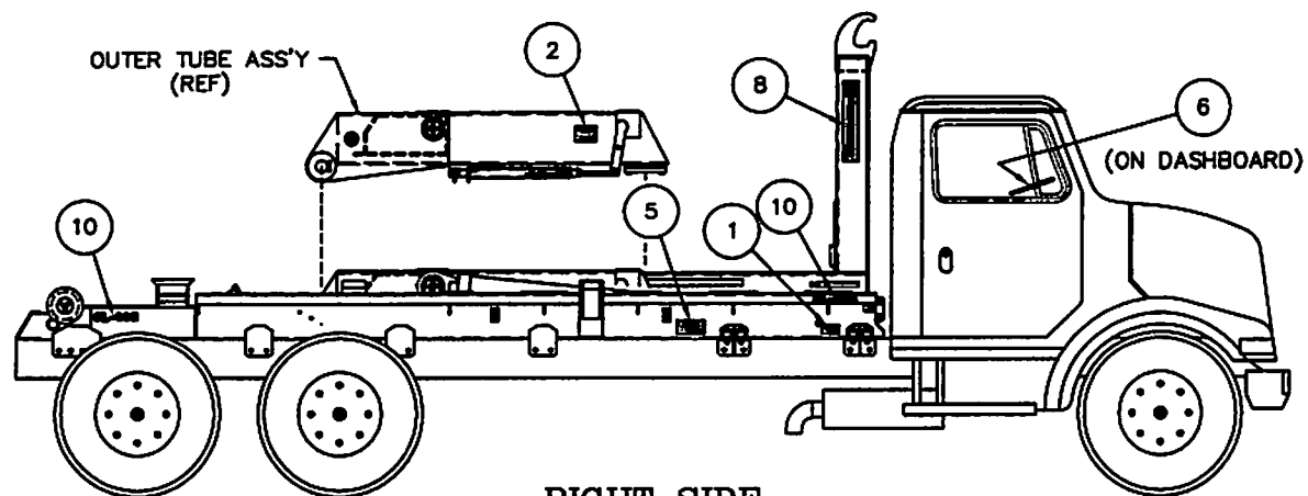
RIGHT SIDE
