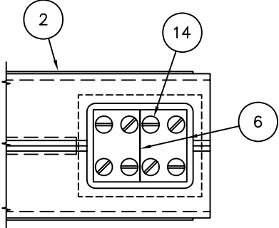
DETAIL C-C
